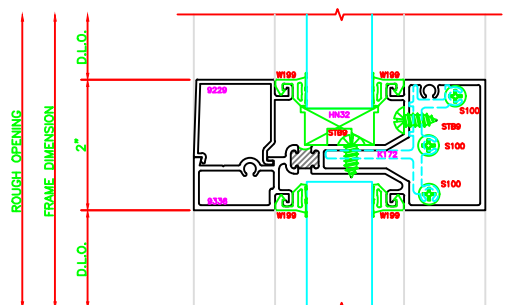
503 O.G. HORZ. 403 SHEARBLOCK
