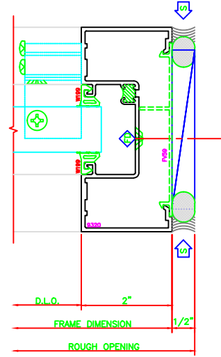
403 JAMB 403 SHEARBLOCK
