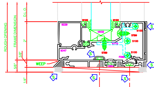
203 O.G. SILL 403 SHEARBLOCK
